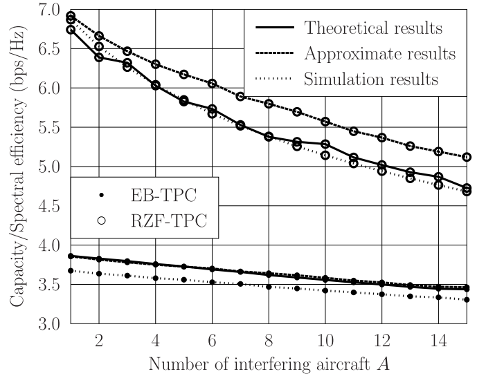
Fig. 4. The achievable throughput per DRA as the function of the number of interfering aircraft A . The distances between the interfering aircraft and the desired receiving aircraft are uniformly distributed within the range of [d_{b^*}^{a^*}, D_{\text{max}}] , and the rest of the parameters are specified in Table III.
