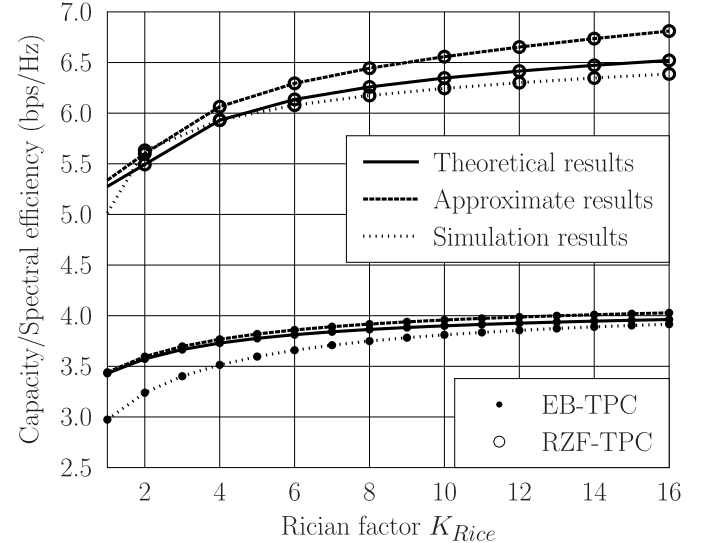
Fig. 9. The achievable throughput per DRA as the function of the Rician factor K_{Rice} . The distances between the interfering aircraft and the desired receiving aircraft are uniformly distributed within the range of [d_{b^*}^a, D_{\max}] , and the rest of the parameters are specified in Table III.
