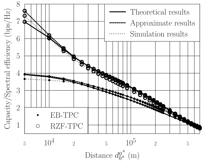
Fig. 5. The achievable throughput per DRA as a function of the distance d_{b^*}^{a^*} between the communicating aircraft a^* and b^* . The distances between the interfering aircraft and the desired receiving aircraft are uniformly distributed within the range of [d_{b^*}^{a^*}, D_{\text{max}}] , and the rest of the parameters are specified in Table III.
