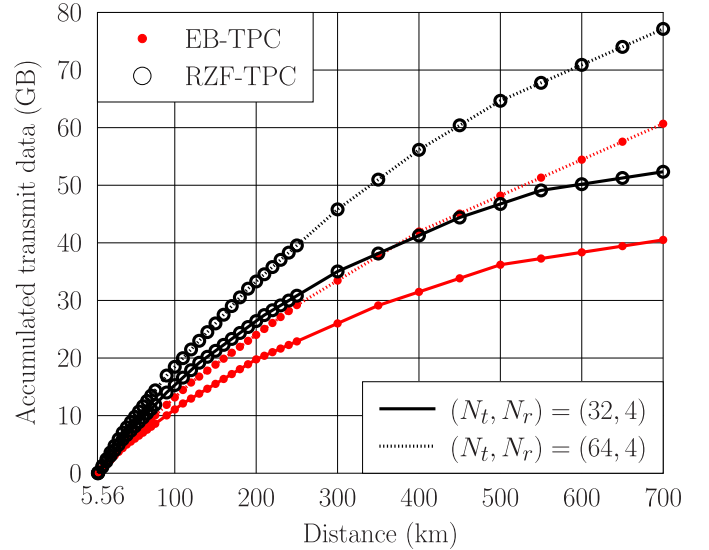
Fig. 3. The accumulated transmitted data volume as the function of the distance d_{b^*}^{a^*} between communicating aircraft a^* and b^* . The distances between the interfering aircraft and the desired receiving aircraft are uniformly distributed within the range of [d_{b^*}^{a^*}, D_{max}] , and other system parameters are specified in Table III.
