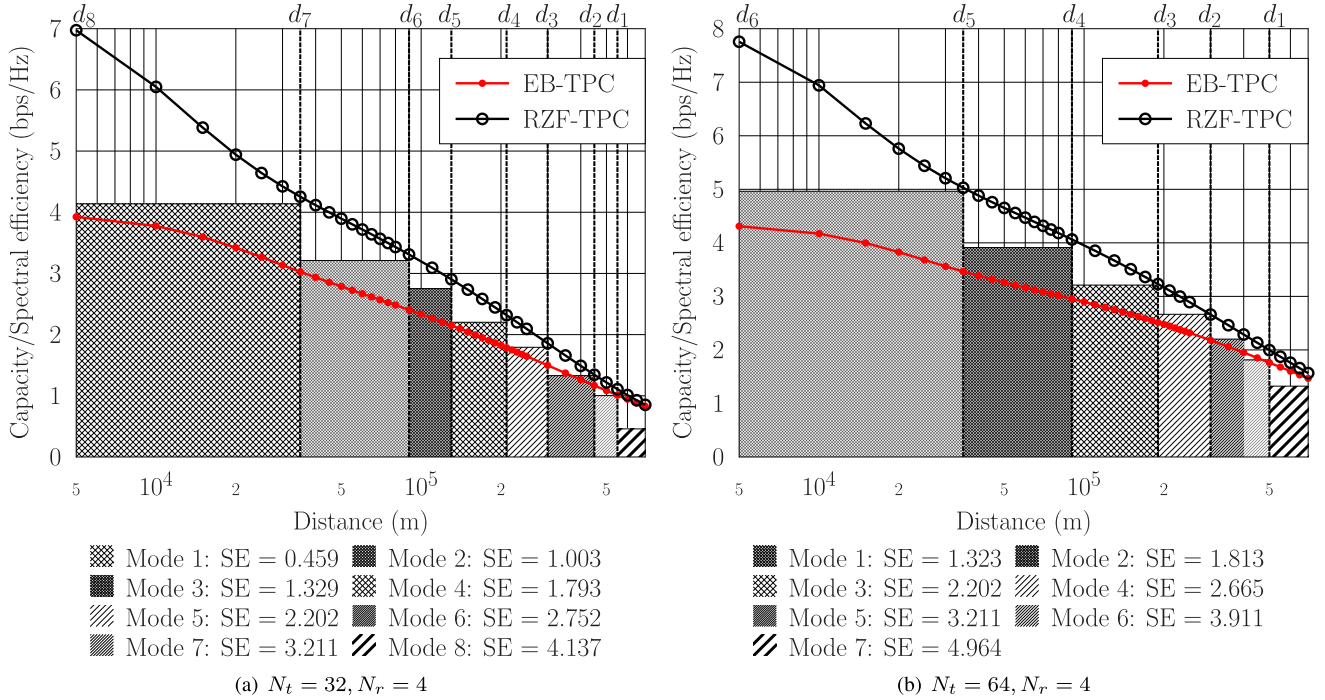
Fig. 2. Two examples of designing the RZF-TPC aided and distance-based ACM scheme. The switching thresholds and achievable system throughputs for (a) and (b) are listed in Tables I and II, respectively.
