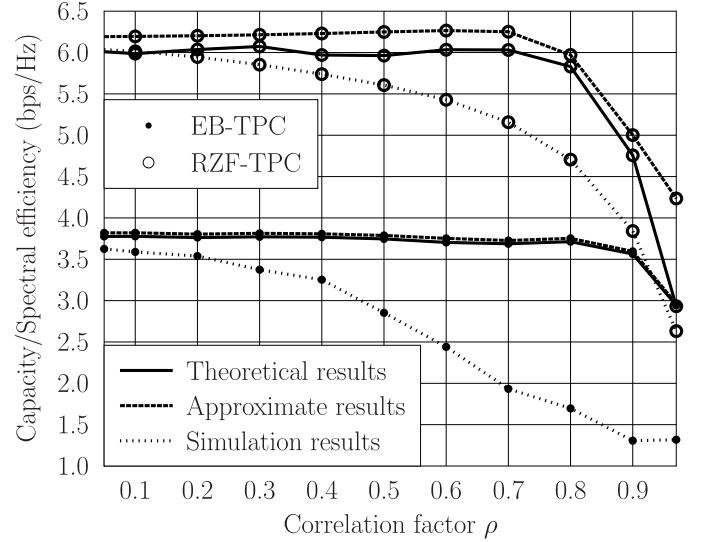
Fig. 8. The achievable throughput per DRA as the function of the correlation factor of DTAs \rho . The distances between the interfering aircraft and the desired receiving aircraft are uniformly distributed within the range of [d_{b^*}^a, D_{\max}] , and the rest of the parameters are specified in Table III.
