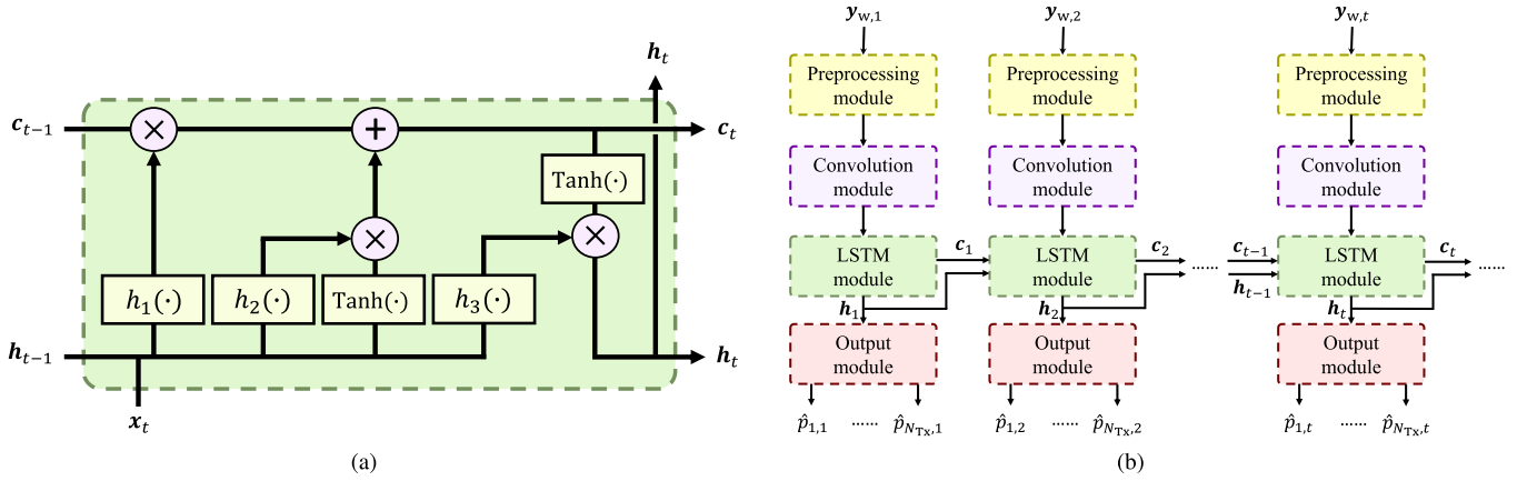
Fig. 3. (a) Basic structure of LSTM, where h_1(\cdot) , h_2(\cdot) and h_3(\cdot) denote hidden layers. (b) Proposed LSTM based model.
