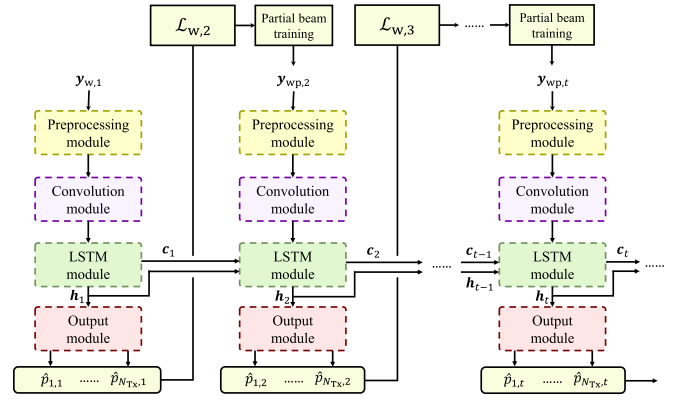
Fig. 4. Proposed adaptive calibrated beam training model.
