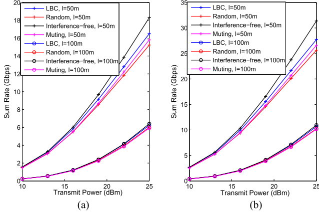
Fig. 9. Network sum rates with m=2 , l=50 m and l=100 m. (a) Scenario A, and (b) Scenario B.
