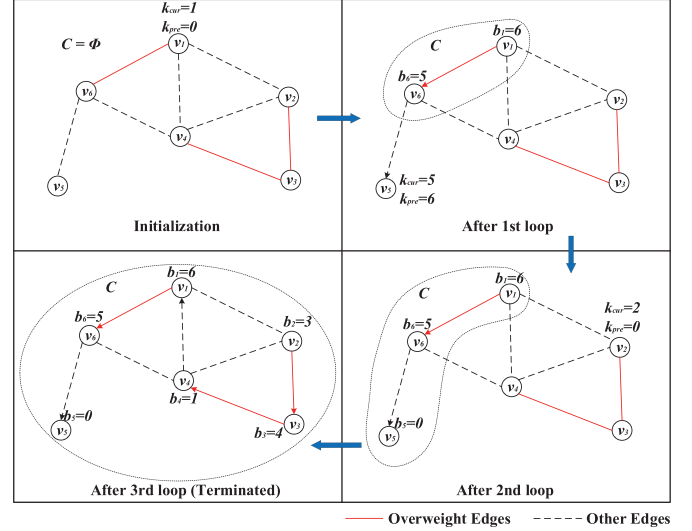
Fig. 3. An example of Algorithm 2 with K = 6 cells. After initialization, the algorithm executes 3 loops and is terminated when C = V . The arrow from one node pointing towards another node indicates that the beam used by the source node may interfere with the destination node of the arrow.
