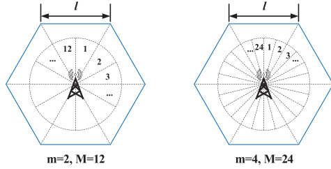
Fig. 4. Beam pattern in a cell. The number of beams in each 60^\circ sector is m = 2, 4 and the total number of beams is M = 12, 24 .
