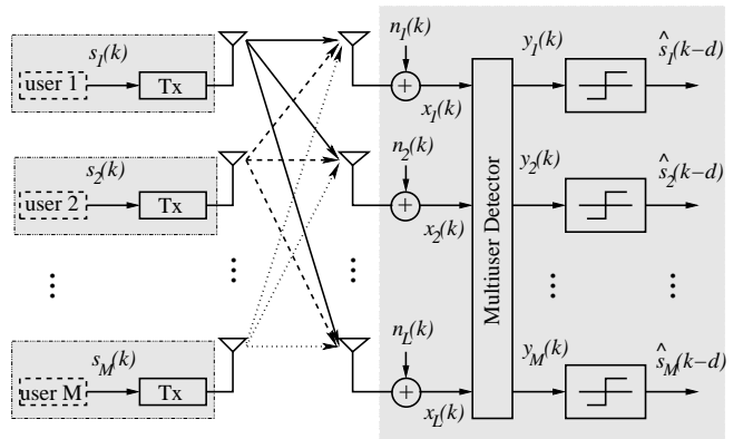
Fig. 1. Schematic of an antenna array aided SDMA uplink scenario, where each of the M users is equipped with a single transmit antenna and the base station's receiver is assisted by an L -element antenna array.
